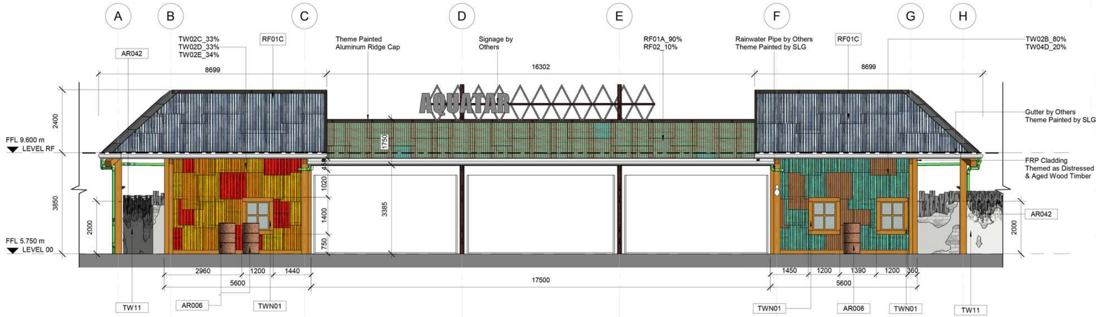
1 ELEVATION 1 0025-04 SCALE 1:75
